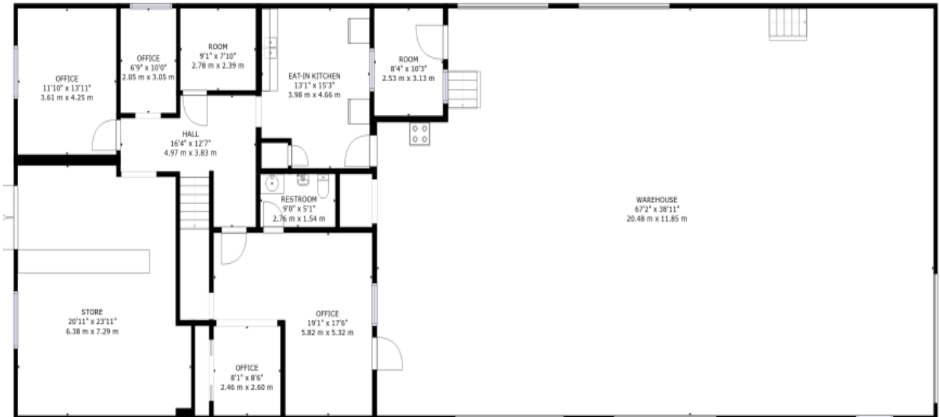
FLOOR 1
